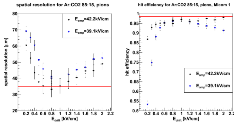
Figure 2: Left: Spatial resolution of conventional micromegas detectors with 250 \mu\text{m} strip pitch as a function of drift-field. Right: hit efficiency as a function of drift-field, both for Ar:CO2 85:15. The inefficiency of about 1.1 % is due to the insensitive area of the insulating pillars keeping the mesh 128 \mu\text{m} above the anode. The efficiency drop above E_{\text{drift}} > 1 \text{ kV/cm} is due to reduced electron transparency of the mesh at E_{\text{amp}} = 39.1 \text{ kV/cm}
