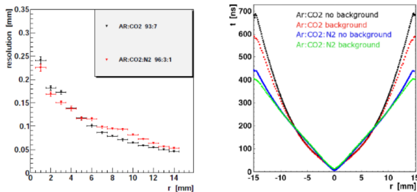
Figure 4: Measurement at the Gamma Irradiation Facility (GIF) at CERN: Left: radial dependent position resolution for both gases without background. Right: rt-reaction for both gases with and without background.
