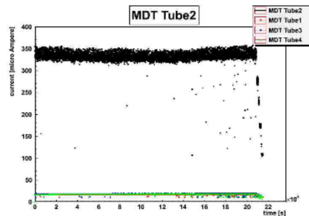
Figure 5: Current in a 30 mm drift tube irradiated with 105 nA of 20 MeV protons over 6 h. The step function at the end of the run corresponds to the intensity of the proton beam decreased stepwise for calibration purposes.
