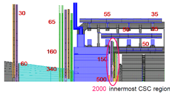
Figure 1: Simulated background induced hit-rate-densities [ \frac{\text{Hz}}{\text{cm}^2} ] in one quarter of the muon spectrometer [5]. The Small Wheel region is encircled in red.
